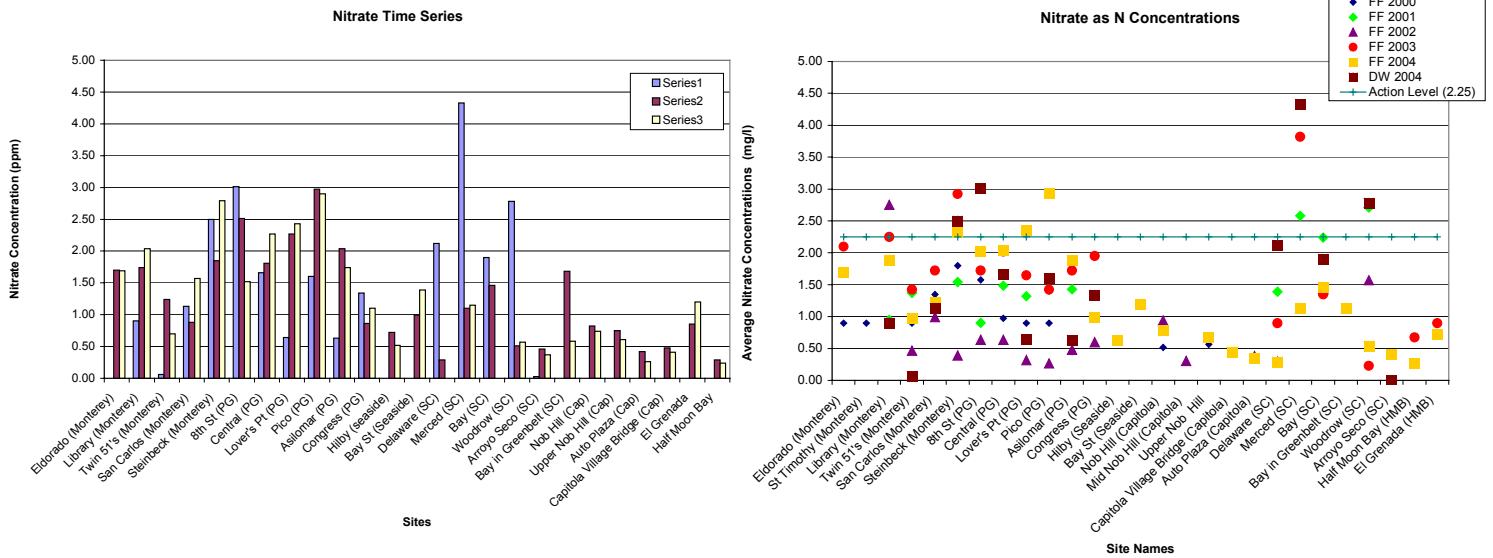
Figure 1. The sites are grouped by city across the bottom. The CCAMP informal action level for nitrate as nitrogen is 2.25 mg-N/l. (1a) Graph of nitrate as nitrogen concentrations in the First Flush 2004 time series. The first column (Series 1) represents the dry weather sample taken, the second series represents the First Flush sample and each subsequent column represents the time series samples, usually taken 30 minutes apart. (1b) Graph of 5-year trend. Average concentrations are represented.
