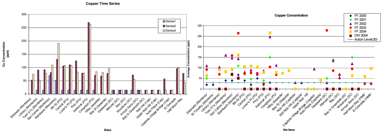
Figure 5. The sites are grouped by city. The Basin Plan Water Quality Objective copper is 30 µg/l. (5a) Graph of copper concentrations in a time series. The first column (Series 1) represents the dry weather sample taken, the second series represents the First Flush sample and time series samples, usually taken 30 minutes apart. (5b) Graph of 5-year trend. Average concentrations are represented.
