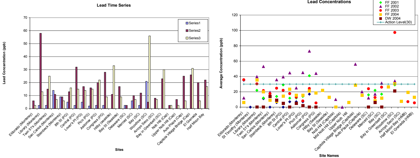
Figure 6. The sites are grouped by city. The Basin Plan Water Quality Objective for lead is 30 µg/l. (6a) Graph of lead concentrations in a time series. The first column (Series 1) represents the dry weather sample taken, the second series represents the First Flush sample and time series samples, usually taken 30 minutes apart. (6b) Graph of 5-year trend. Average concentrations are represented.
