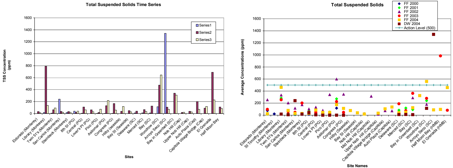
Figure 8. The sites are grouped by city. The CCAMP action level for TSS is 500 mg/l. (8a) Graph of total suspended solid concentrations in a time series. The first column (Series 1) represents the dry weather sample taken, the second series represents the First Flush sample and time series samples, usually taken 30 minutes apart. (8b) Graph of 5-year trend. Average concentrations are represented
